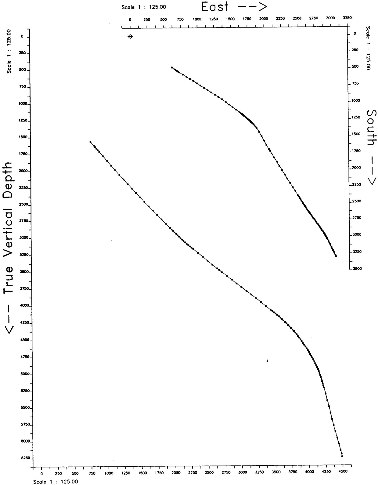
Vertical Section on 137.00 azimuth with reference 0.00 N, 0.00 E from C-239 M1
